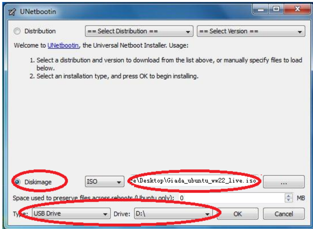
Figure 1 Making USB Live Creator
