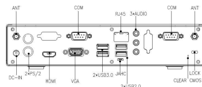
Rear Panel External I/O
