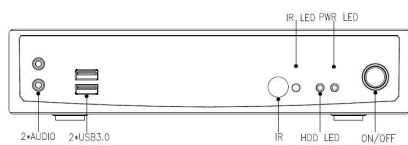
Front Panel External I/O
